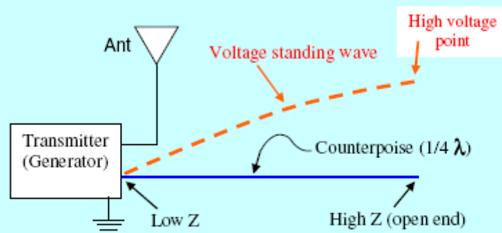
Fig. 6. Voltage standing wave in a quarter wavelength counterpoise
